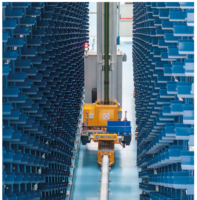
MLB100Q twin-mast stacker crane It can reach up to 20 m high and handle two 100 kg unit loads or four 50 kg unit loads.
