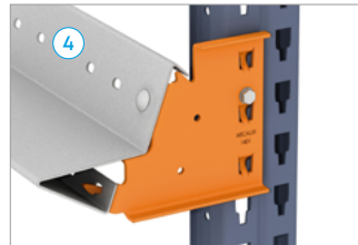
GP rail
