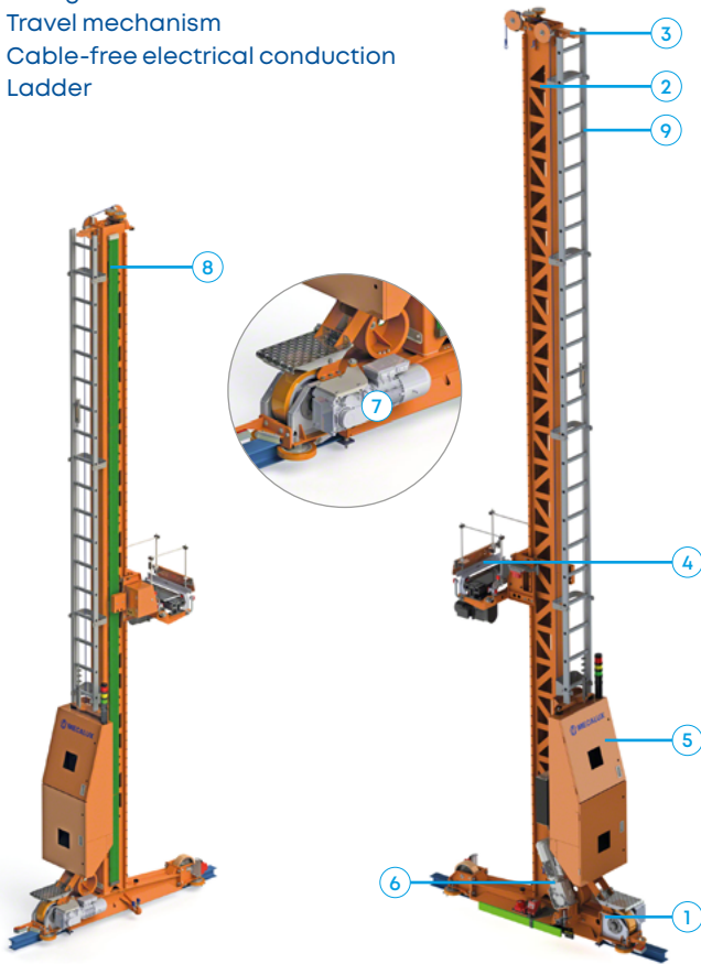
ML50 single-mast stacker crane It can handle a box of up to 50 kg at a height of 9 m.
